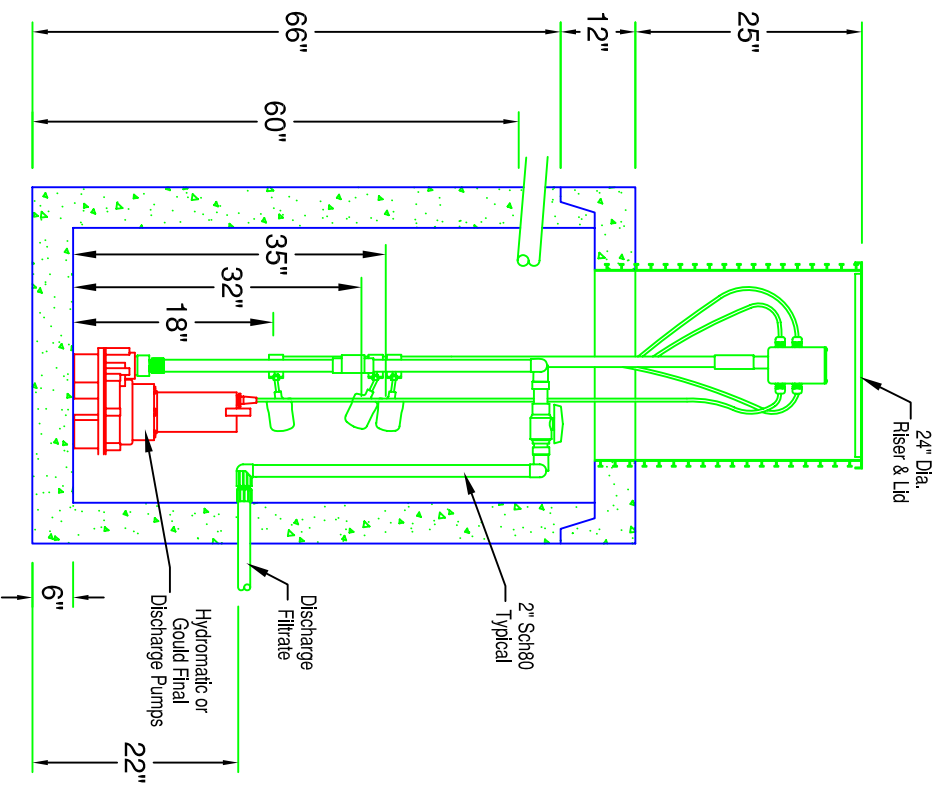
3'-0" Dia. Final Discharge (Low-Head)
