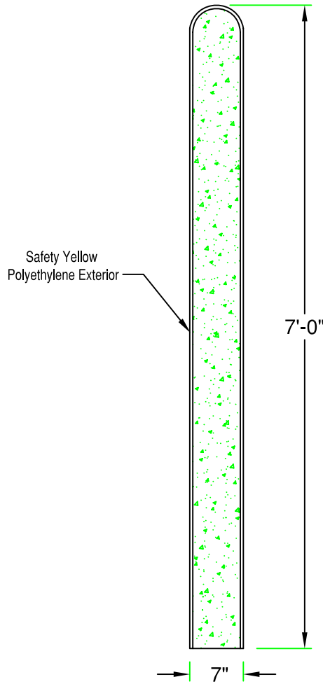
Section
